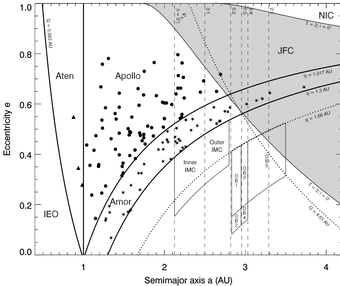
Fig. 1.— NEO figure
