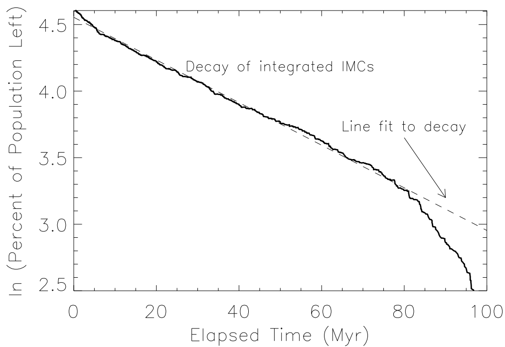
Fig. 9.— Decay of IMC population
