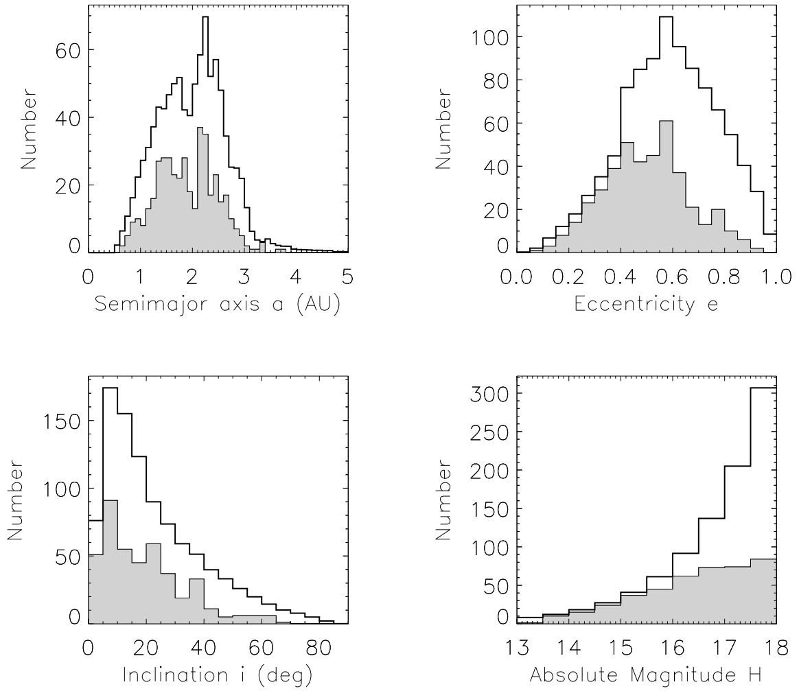
Fig. 12.— Predicted and observed NEOs
