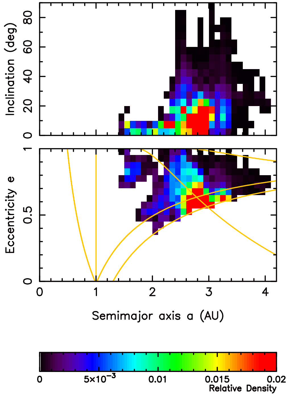
Fig. 6.— Outer main belt (OB)
