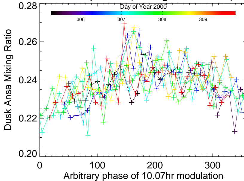
O II Epoch 7 (Strong Modulation)
