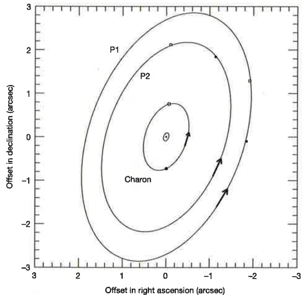
Figure 2 | Preliminary orbits for P1 and P2, assuming that they are circular and in the same plane as Charon's orbit. The barycentre of the system is the dot in the centre, Pluto's orbit is the smallest ellipse, Charon's orbit is the next ellipse (its positions on 15 May and 18 May are indicated by the filled and open circles, respectively), an orbit that is consistent with P2's measured positions is next, followed by an orbit that is consistent with P1's measured positions. For the last two cases, the filled squares are the observed positions on 15 May, and the open squares are the observed positions on 18 May. The uncertainties ( 1\sigma ) in the measured positions are approximately the size of the symbols. At Pluto's distance, 1 arcsec projects to 21,800 km. Charon's orbital plane is inclined by \sim 36^\circ relative to the line-of-sight, which means that the circular orbits of the satellites appear elliptical when projected on the plane of the sky. All four objects orbit the barycentre in an anticlockwise direction in this view, and all positions are displayed in the J2000 reference frame with celestial north up and east to the left.
